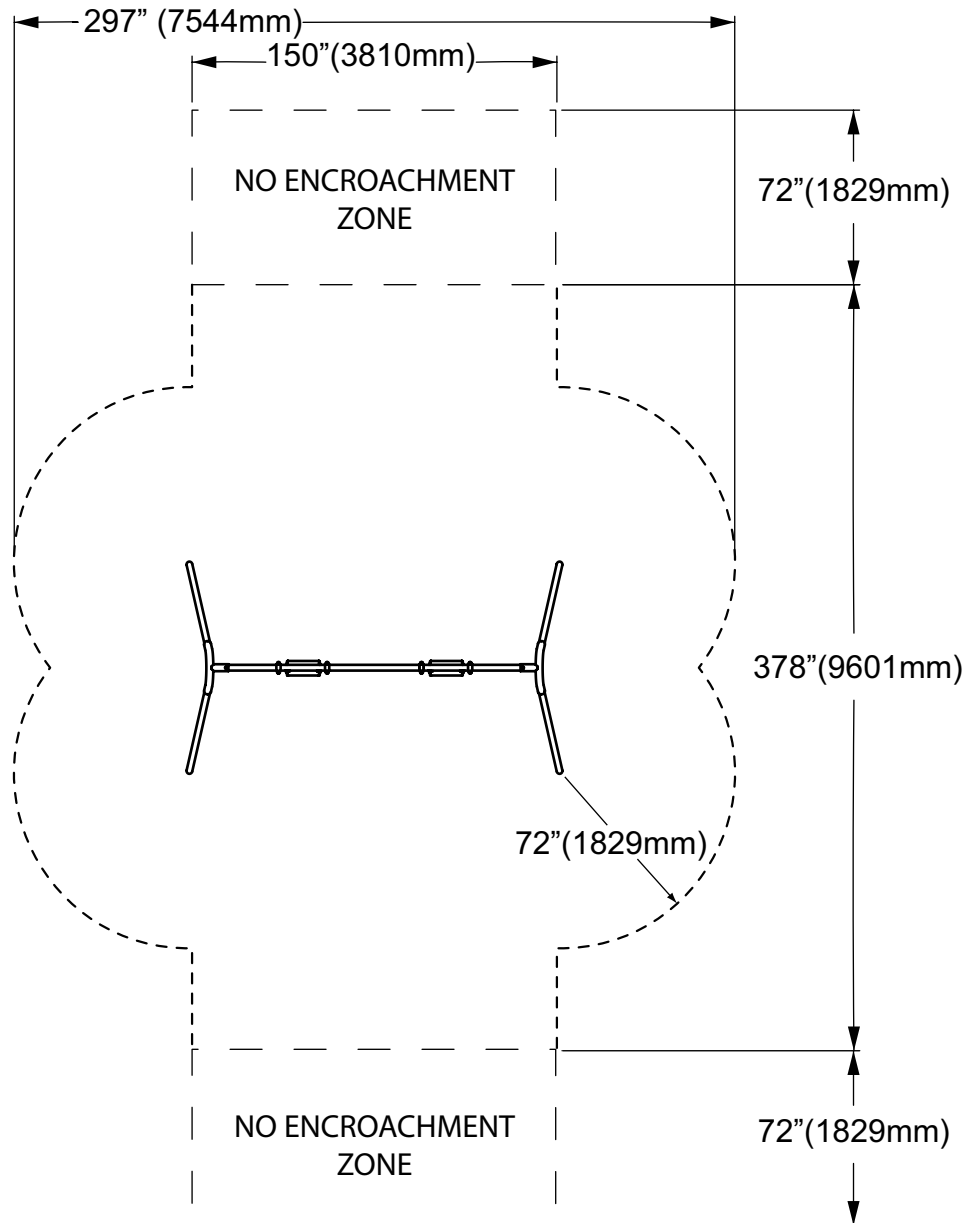
TOP VIEW
