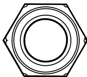
7/16" Lock Nut (33-01-0017)
